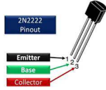
2N2222 pinout
