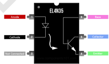
CNY75C and 4N35 pinout
